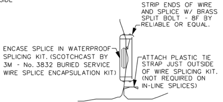
TRACER WIRE SPLICE DETAIL Not to Scale
