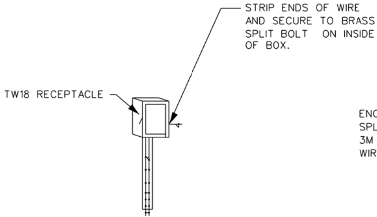
TRACER WIRE RECEPTACLE DETAIL Not to Scale
